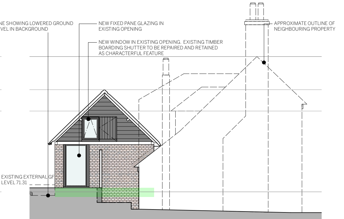
SOUTHWEST (SIDE) ELEVATION
