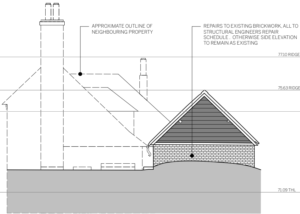
NORTHEAST (SIDE) ELEVATION NEIGHBOURING PROPERTY SIDE
