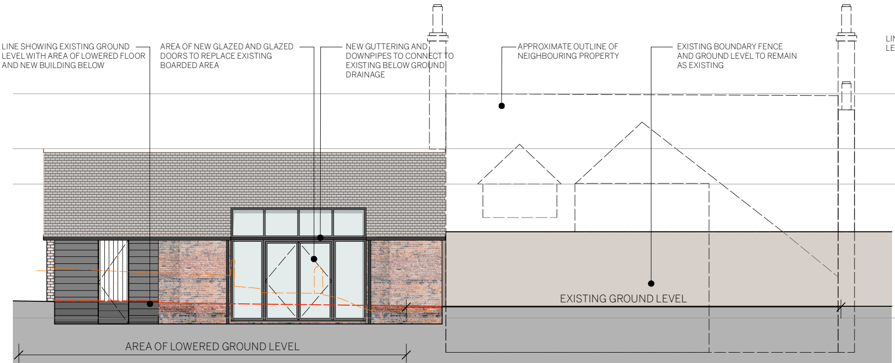
NORTHWEST (FRONT) ELEVATION
