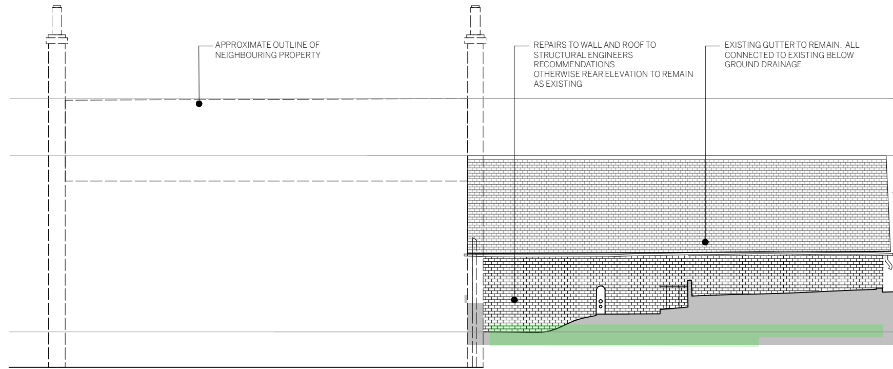
SOUTHEAST (REAR) ELEVATION NEIGHBOURING PROPERTY SIDE
