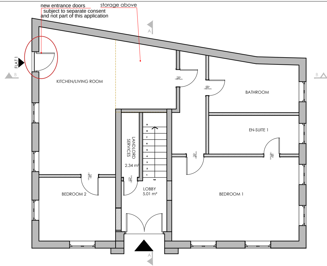
13 PROPOSED GROUND FLOOR PLAN A-(13)-011 1:50@ A1,1:100 @ A3
