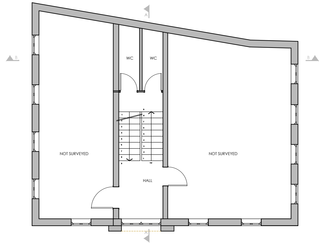
14 PROPOSED SECOND FLOOR PLAN - AS EXISTING A-(13)-011 1:50@ A1,1:100 @ A3
