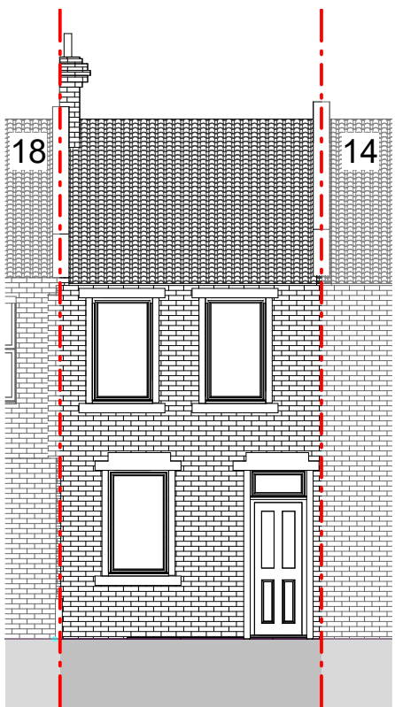
West Elevation - Existing 1 : 100
