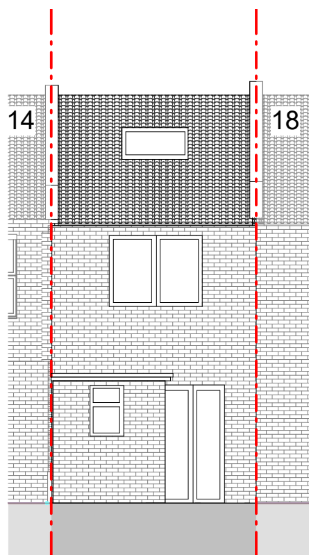
East Elevation - Proposed 1 : 100
