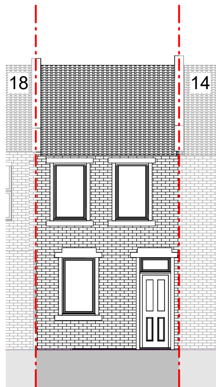
West Elevation - Proposed 1 : 100
