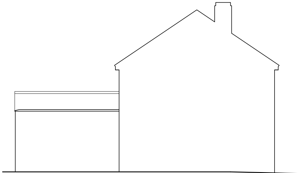
PROPOSED L.H. SIDE ELEVATION
