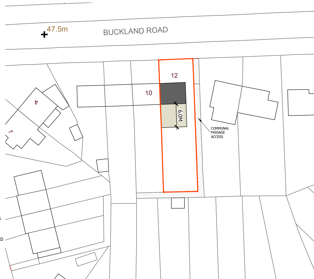
BLOCK PLAN
