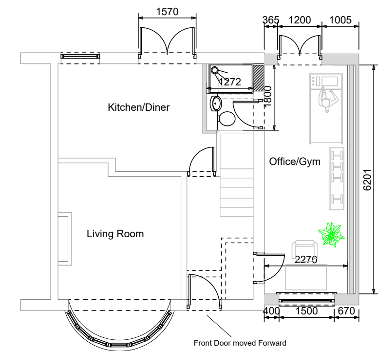
Proposed Ground Floor Layout
