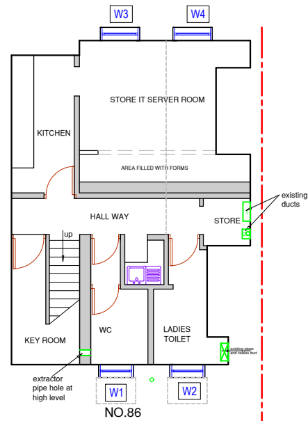
EXISTING BASEMENT FLOOR PLAN
