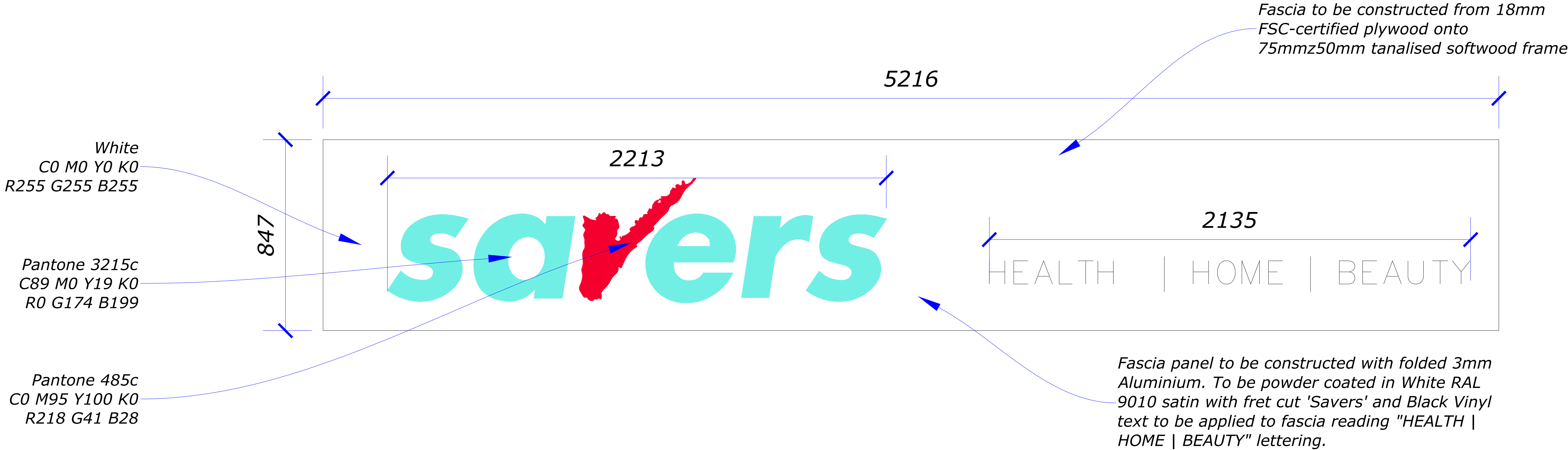
2No. Proposed Internally Illuminated Fascia Signs Scale 1:10 @ A1
