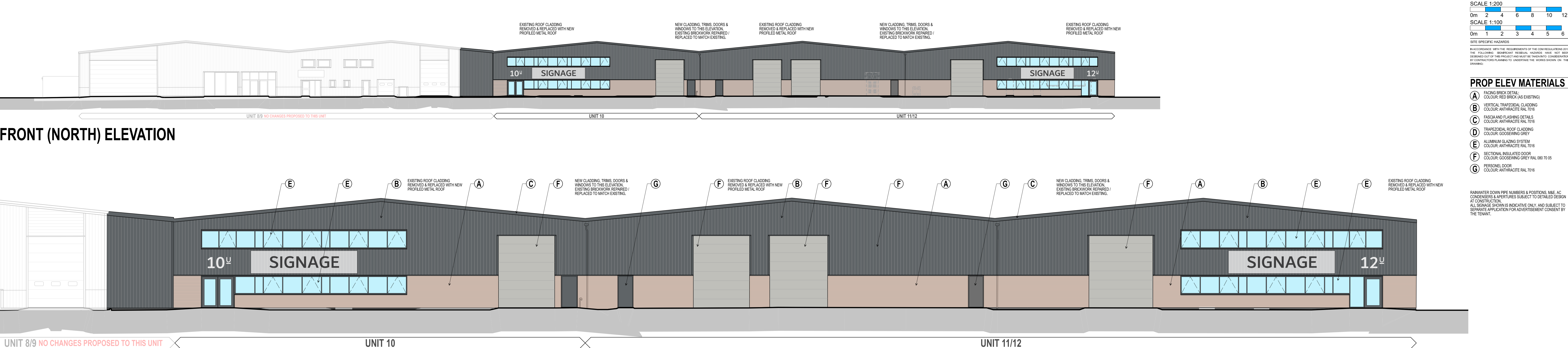
ENLARGED FRONT (NORTH) ELEVATION 1:100
