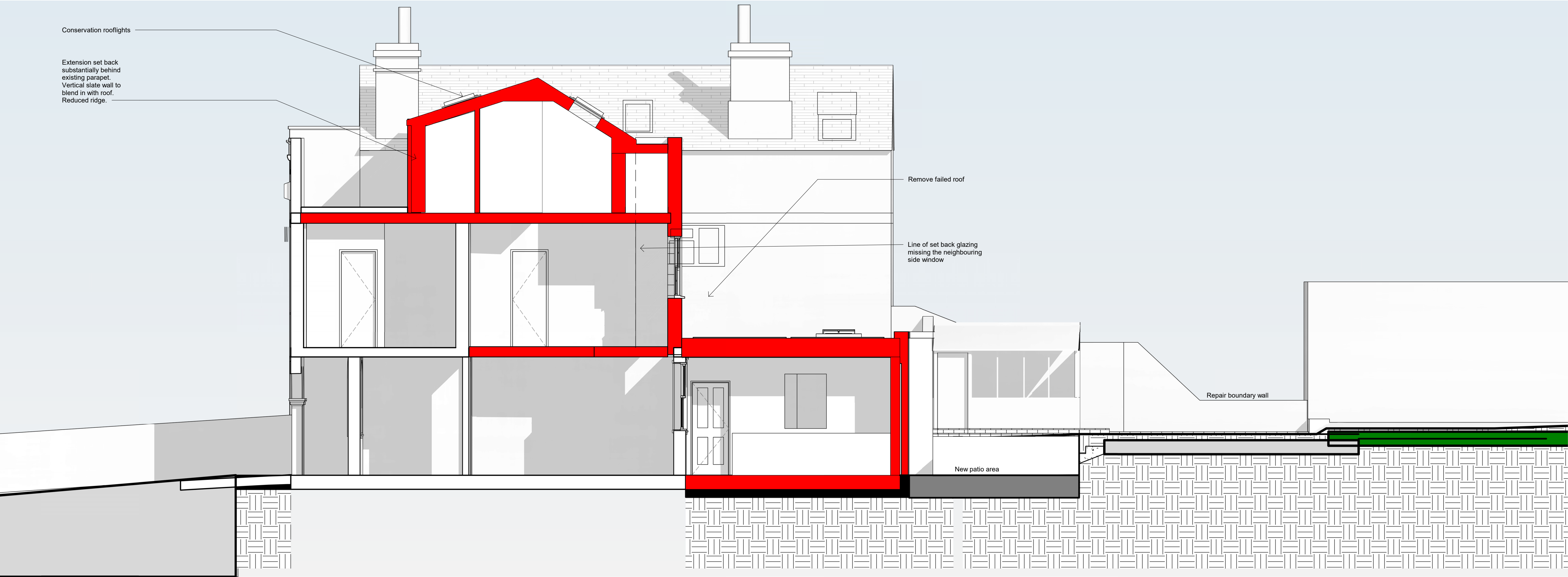
North West -View of adjacent property Proposed 1 : 50
