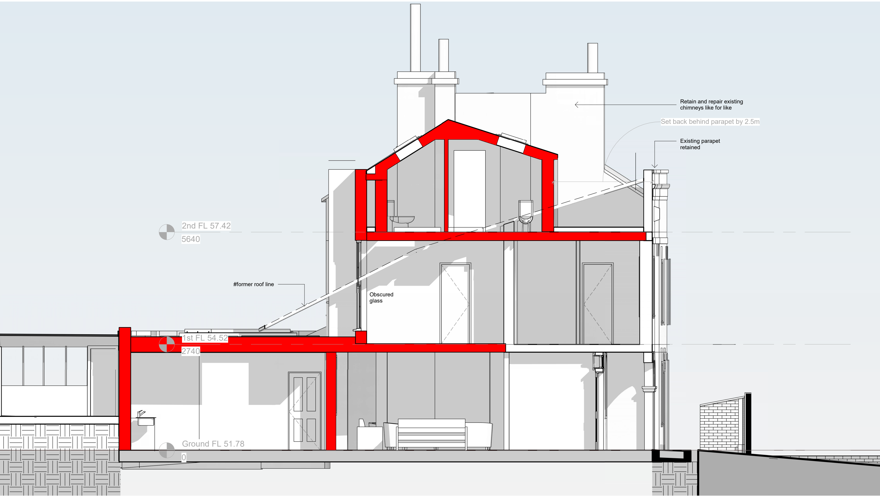
Side Elevation/ Section through Lower Section Proposed 1 : 50
