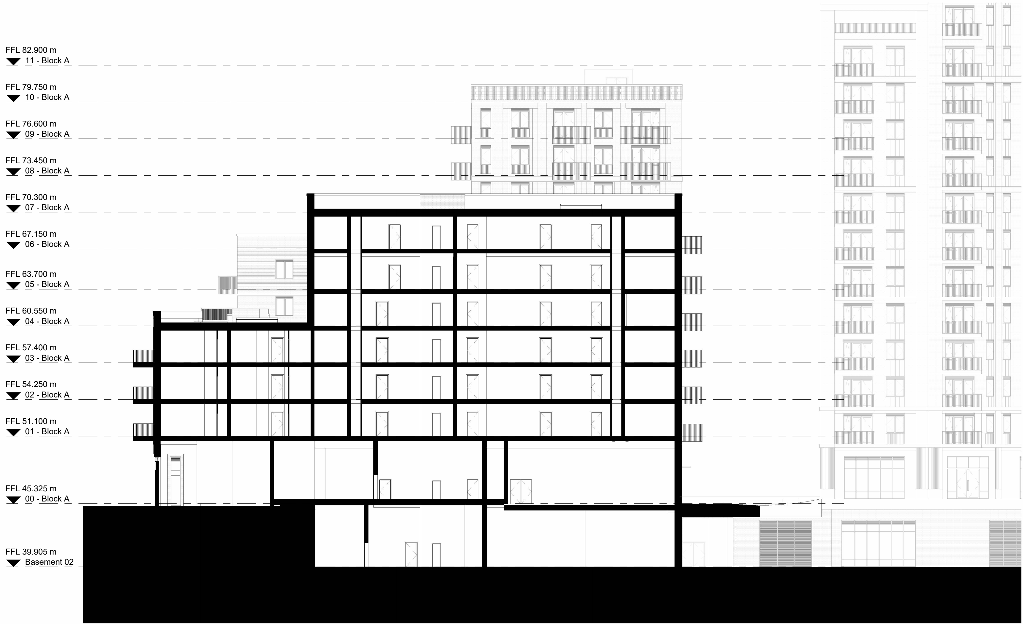
Block A - Section CC 1 : 200
