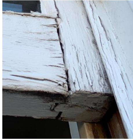
Rot to the lower sash bottom rail and stile joints
