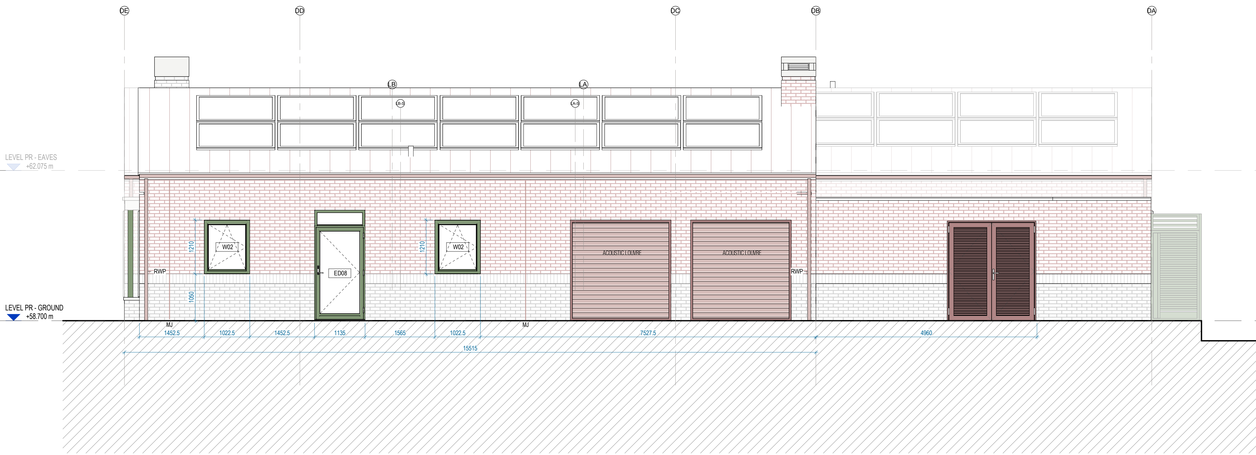
Block D East Elevation 1
