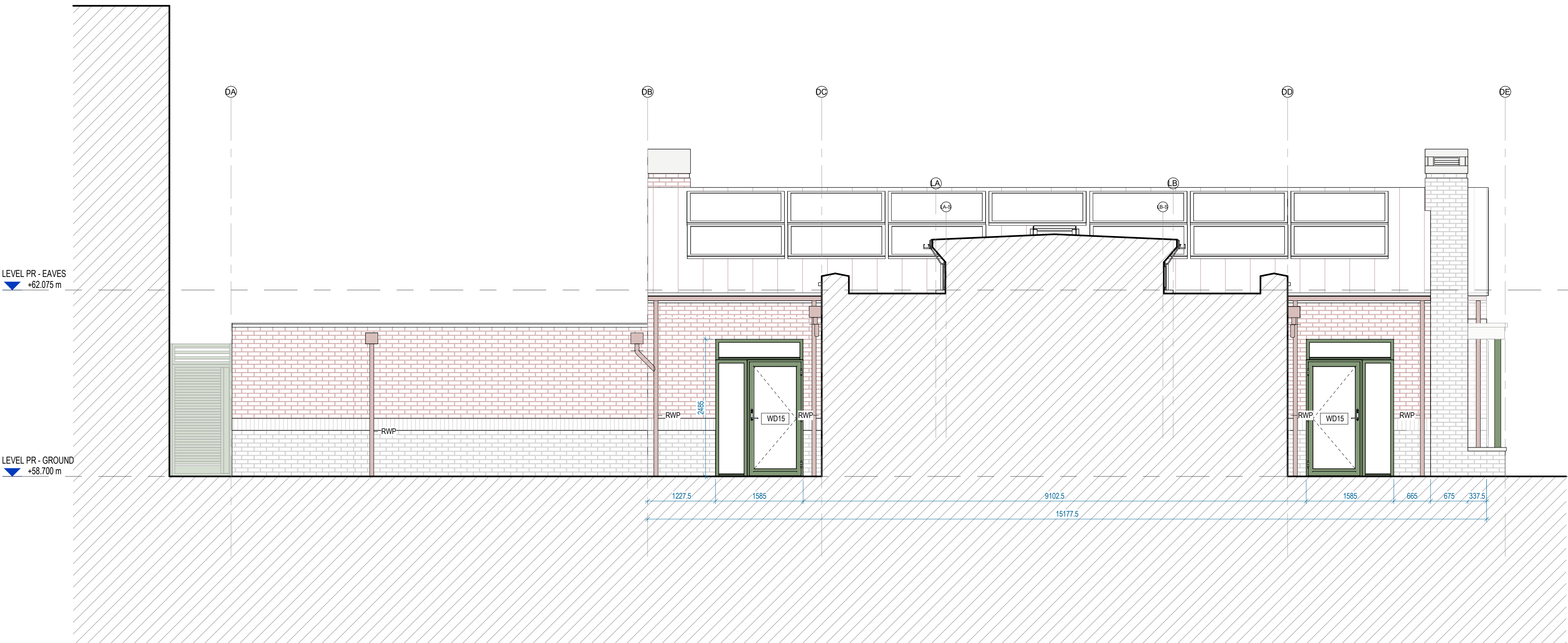
Block D West Elevation 2
