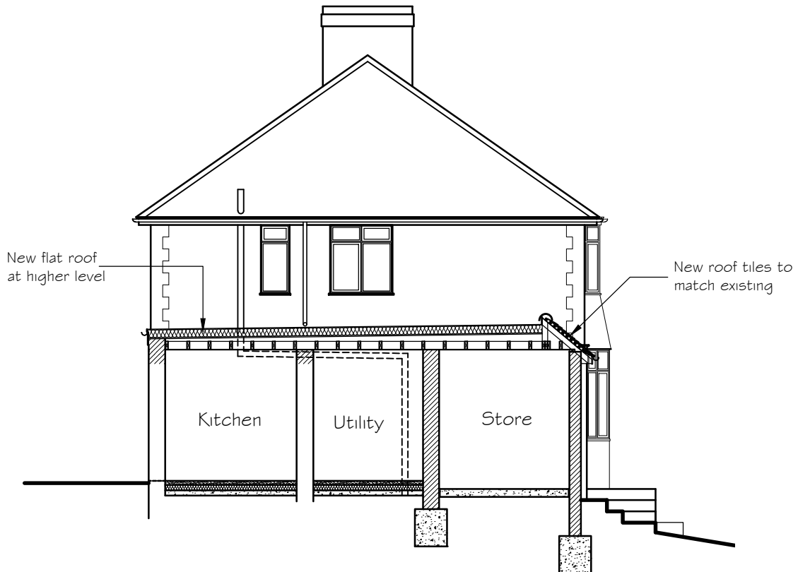
TYPICAL SECTION
