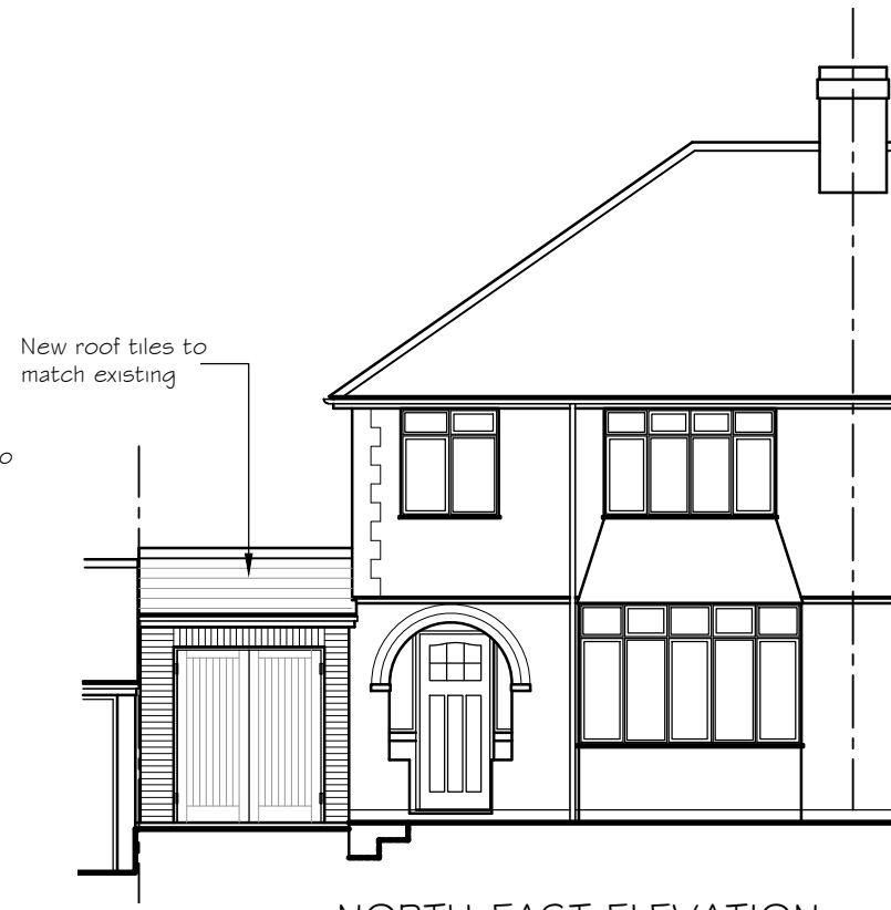
NORTH-EAST ELEVATION
