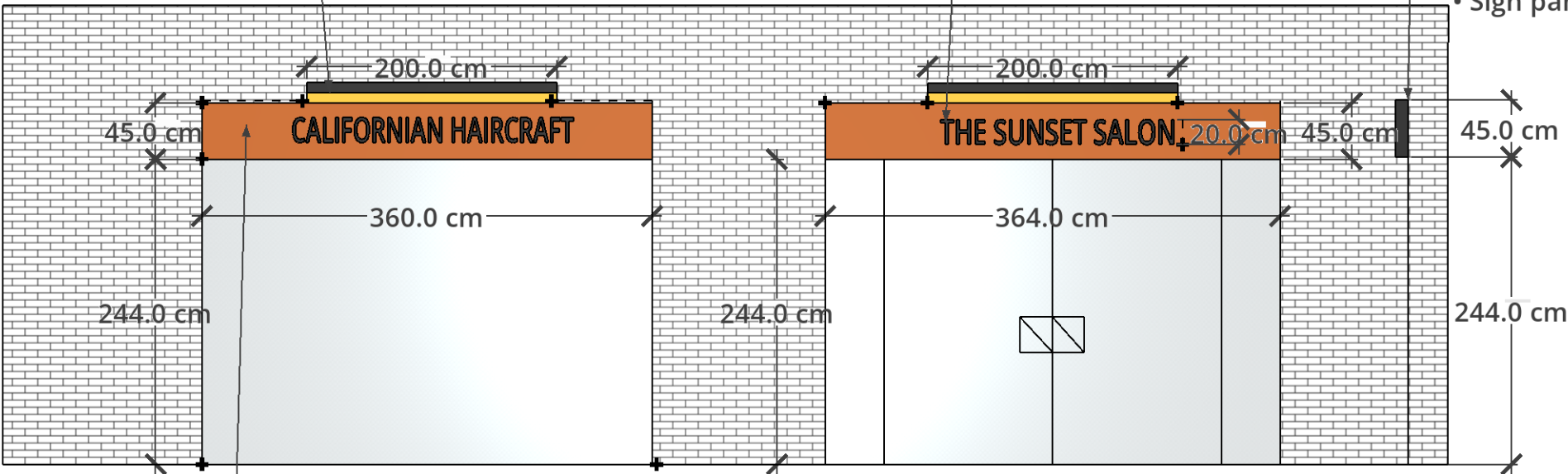
PROPOSED SHOP FRONT ELEVATION
