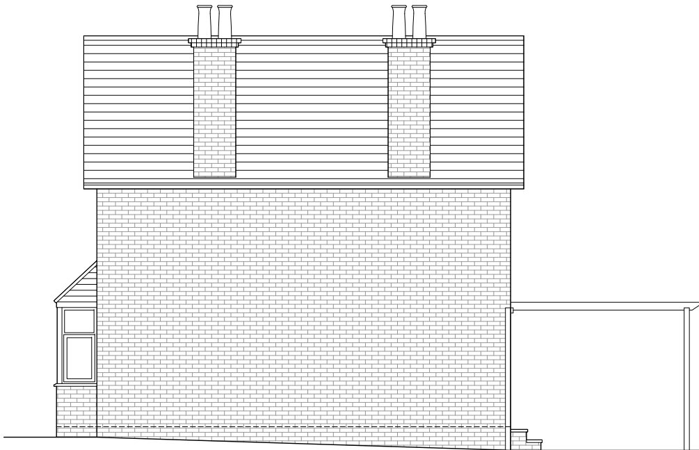
Elevation D
