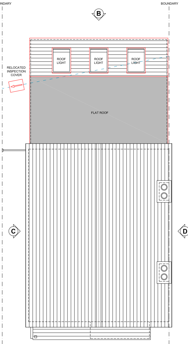
Roof Plan
