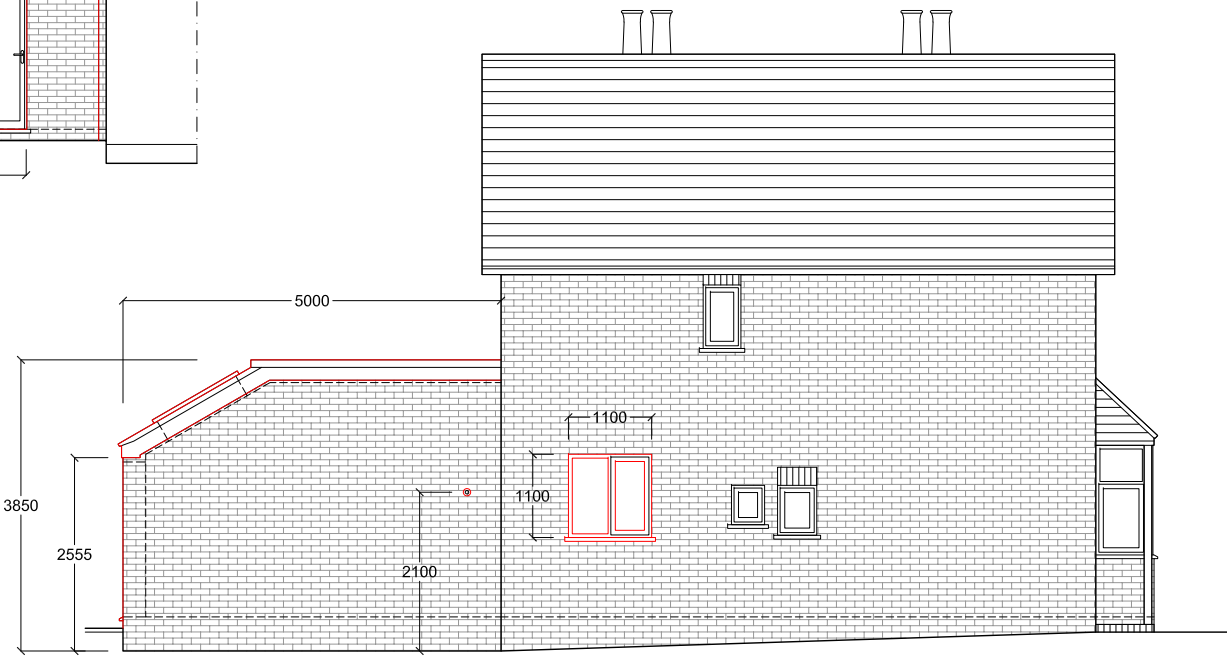
Elevation C
