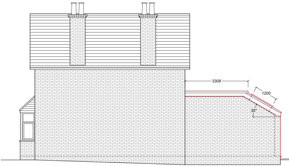
Elevation D
