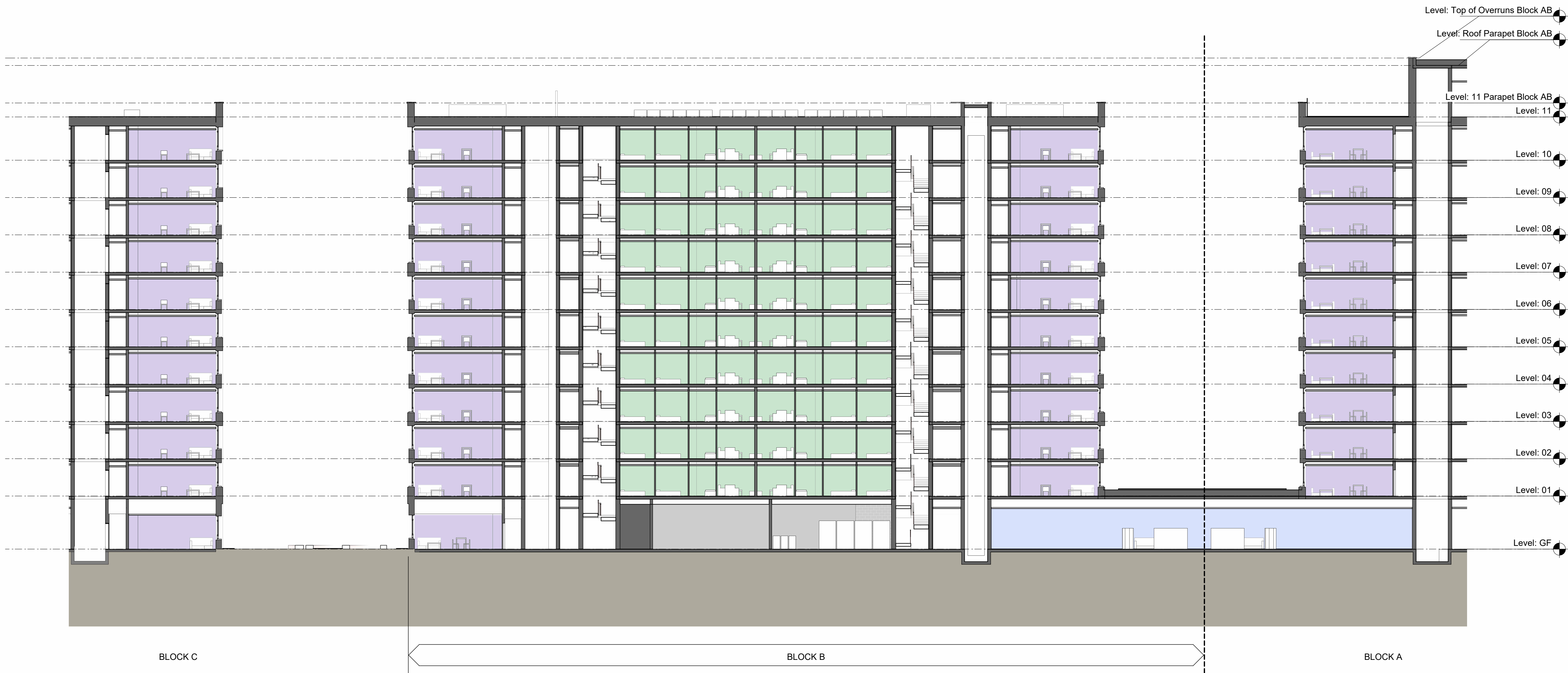
1 BB-05-S-Section-WestToEast 1:200
