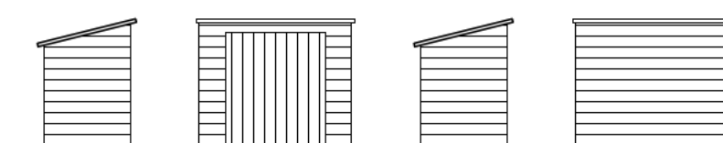
TYPICAL ELEVATIONS OF BIKE AND BIN STORE
