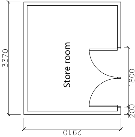
As-Built And Proposed Plan
