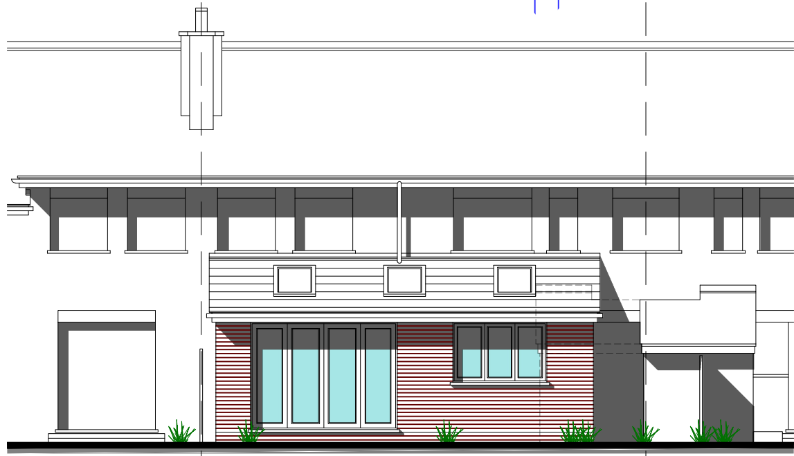
Rear Elevation 1:100 Scale
