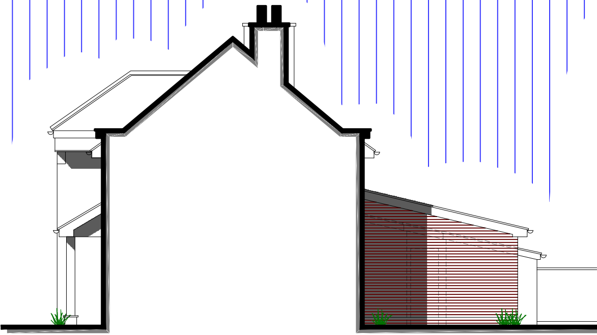
Side Elevation 1:100 Scale
