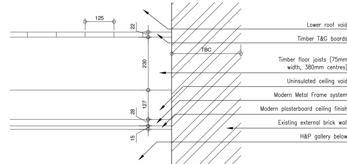
02 RF19 ROOF SPACE FLOOR BUILDUP 1:10
