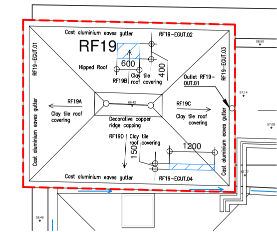
03 EXISTING ROOF PLAN RF19 1:100
