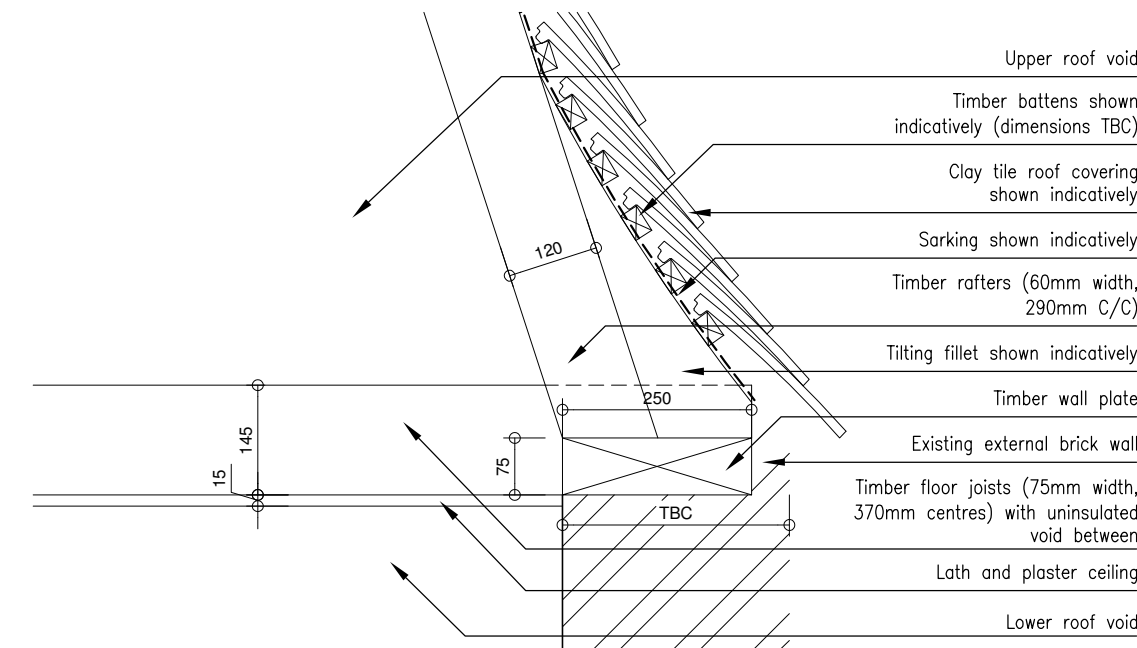
01 RF19 ROOF SPACE CEILING JOISTS AND ROOF RAFTERS 1:10
