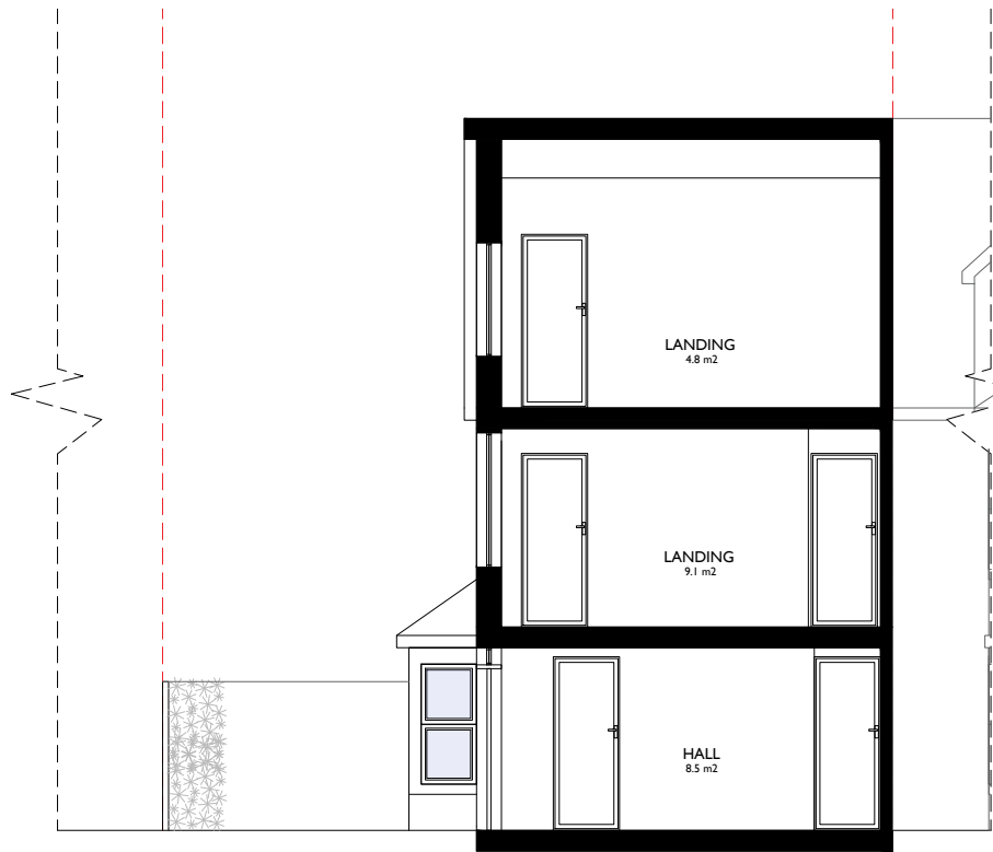
Existing AA Section
