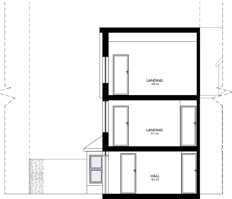
Proposed AA Section
