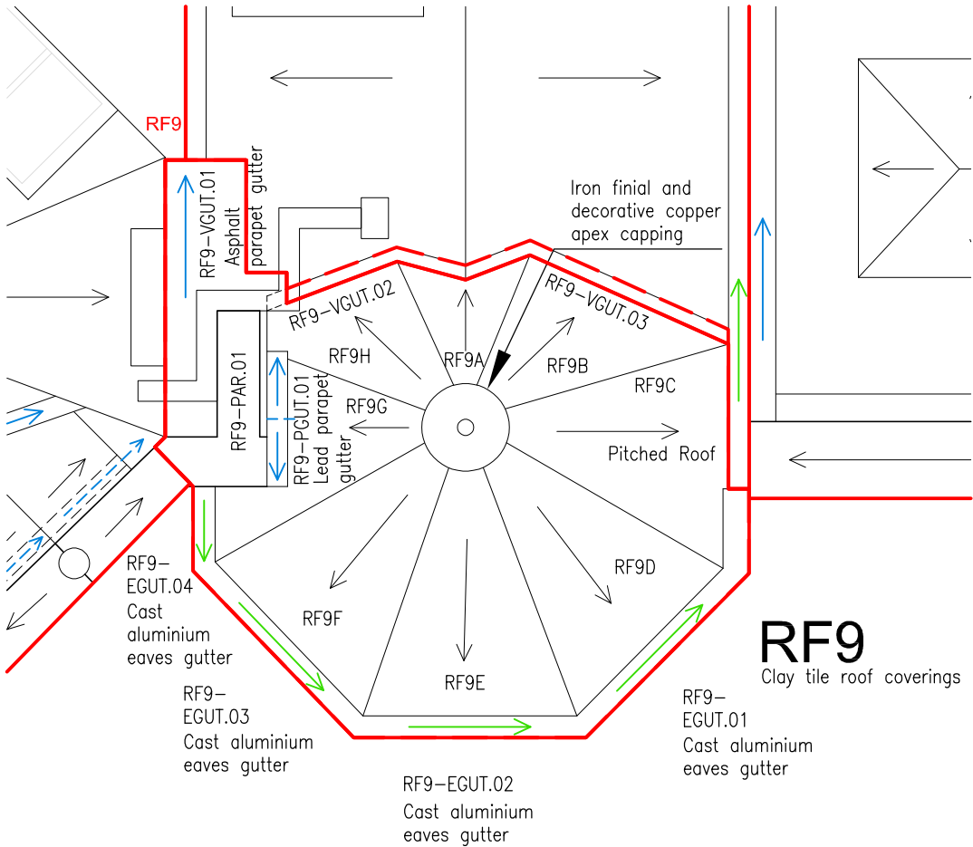
02 EXISTING ROOF PLAN RF9 1:50
