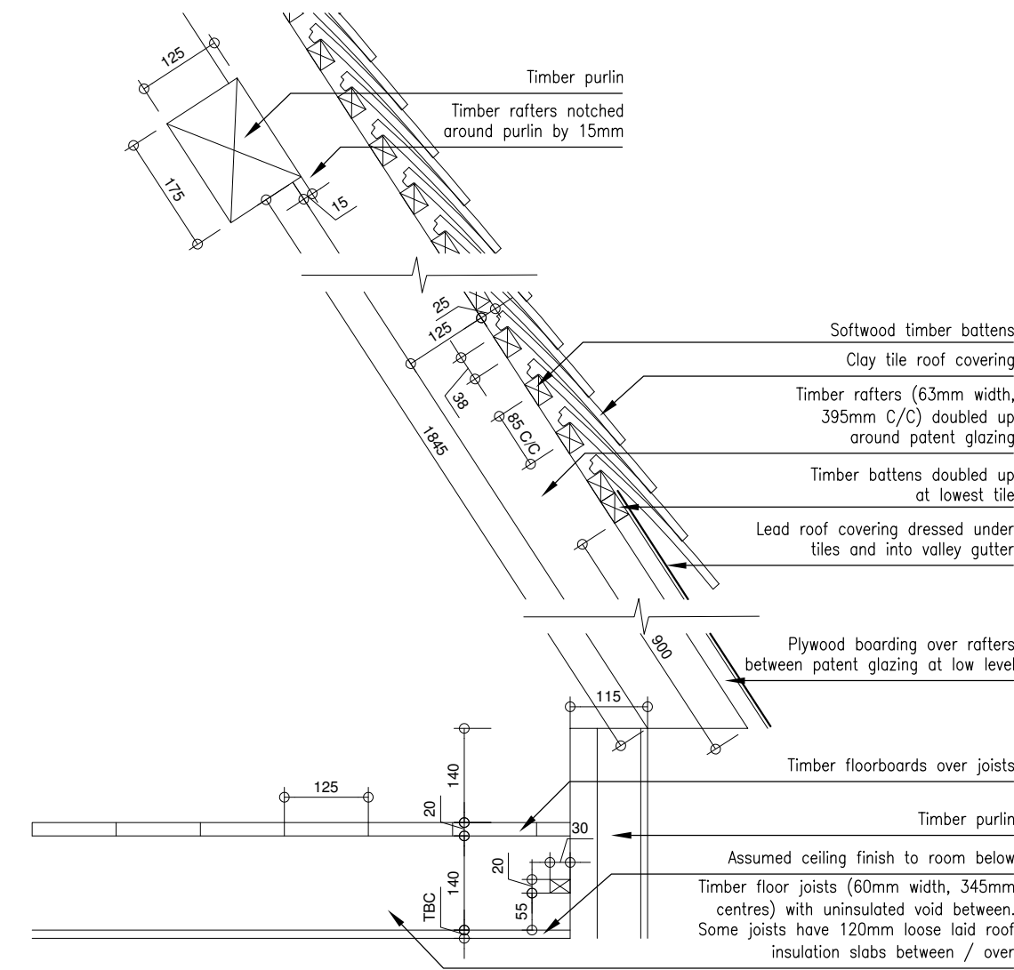
01 RF7 TYPICAL ROOF BUILDUP
