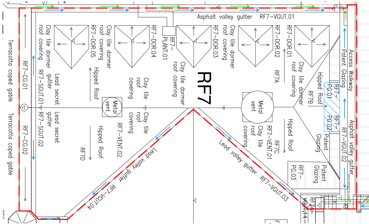
02 EXISTING ROOF PLAN RF7
