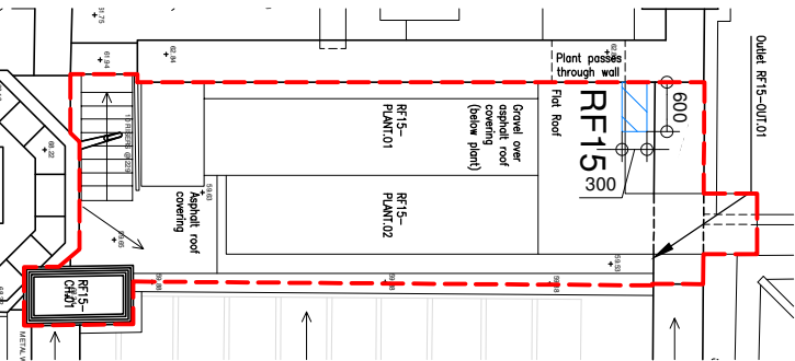
02 EXISTING ROOF PLAN RF15 1:100 Scale Bar. 1:100
