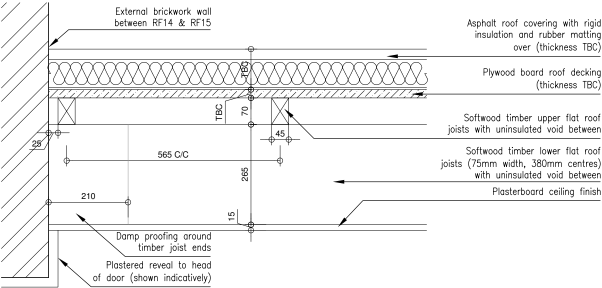
01 RF15 TYPICAL ROOF BUILDUP 1:10 Scale Bar. 1:10
