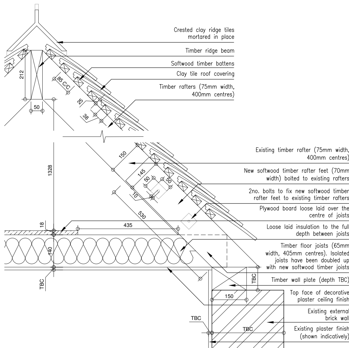
01 RF8 TYPICAL TILED ROOF BUILDUP 1:10
