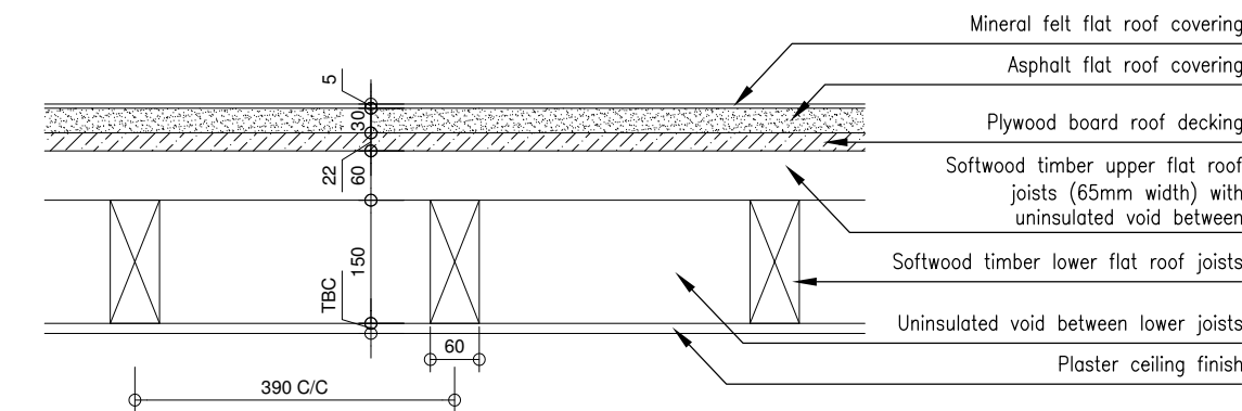
02 RF8 TYPICAL FLAT ROOF BUILDUP 1:10 Scale Bar. 1:10
