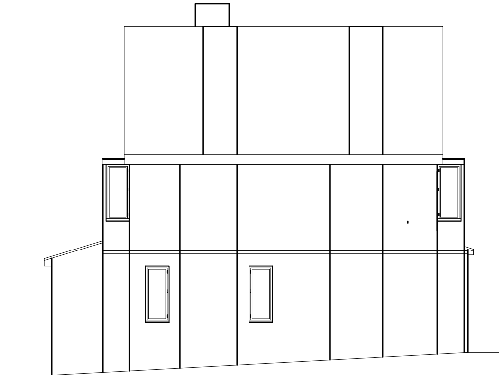
Proposed Side Elev
