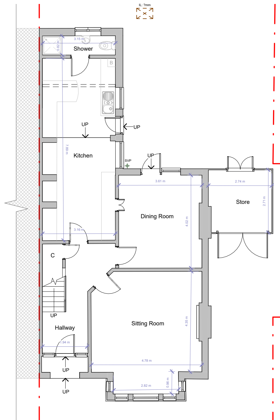
Ground Floor
