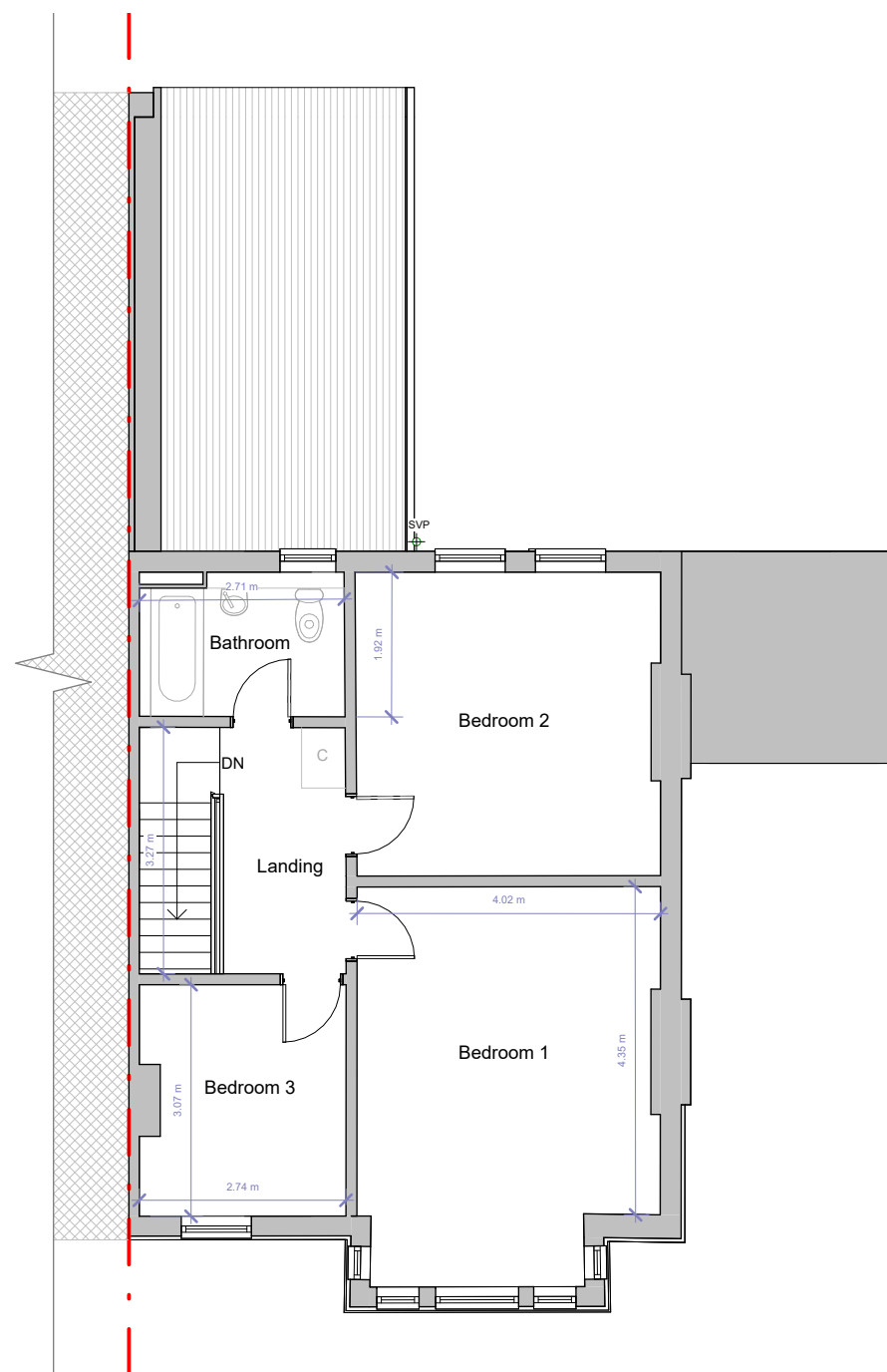
First Floor
