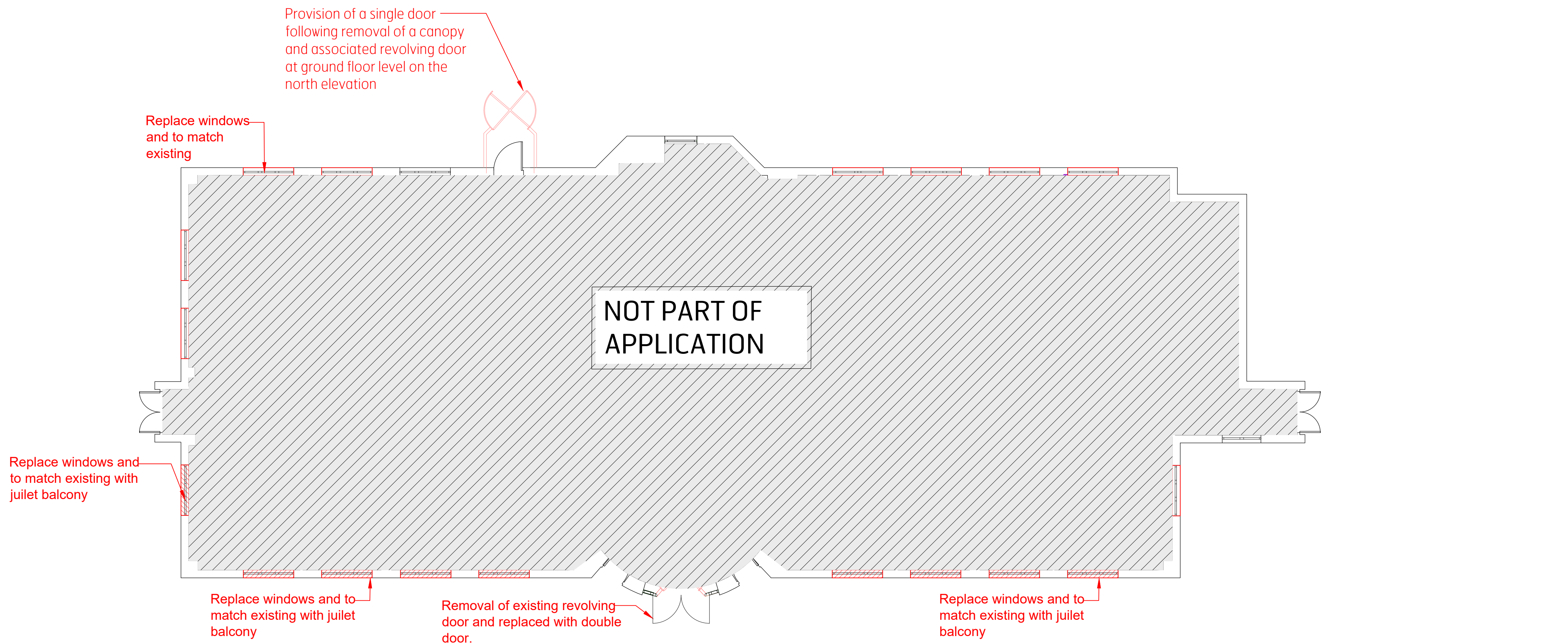
PROPOSED GROUND FLOOR A1@1:100
