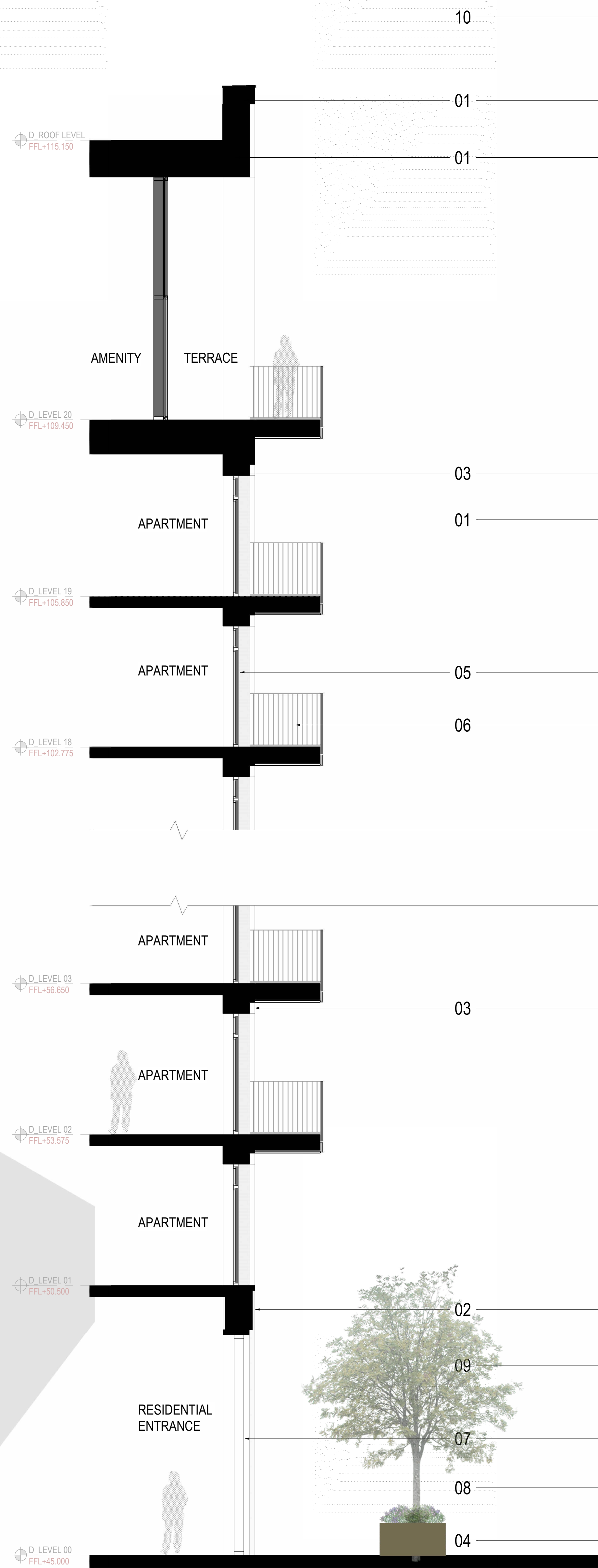
2 PLOT D BAY STUDY SECTION SCALE: 1 : 50
