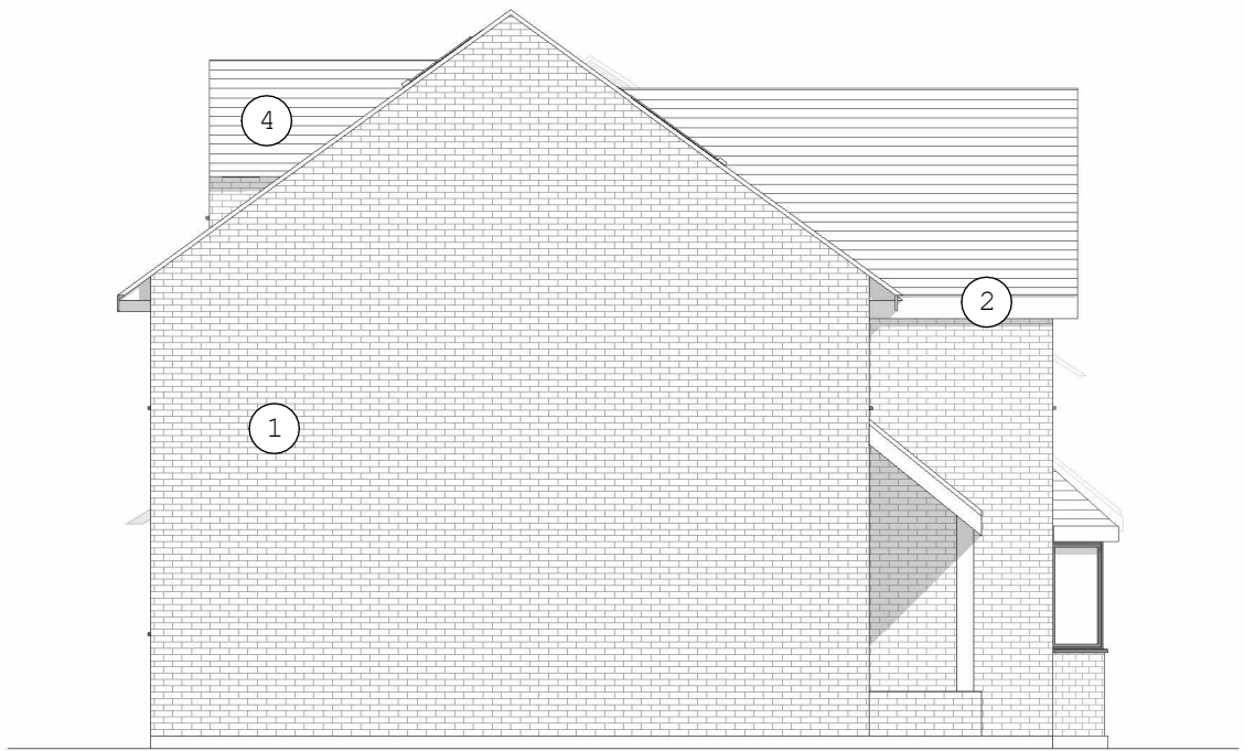
PROPOSED NORTH SIDE ELEVATION
