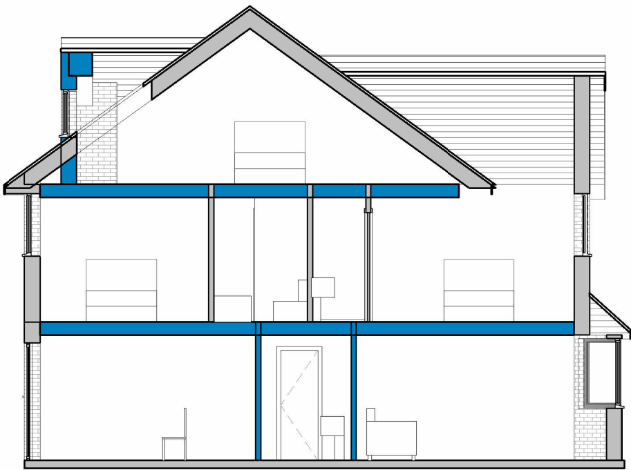
UNIT 1 AND 2 SECTION
