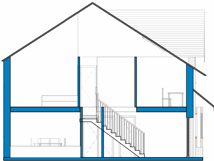
UNIT 3 SECTION
