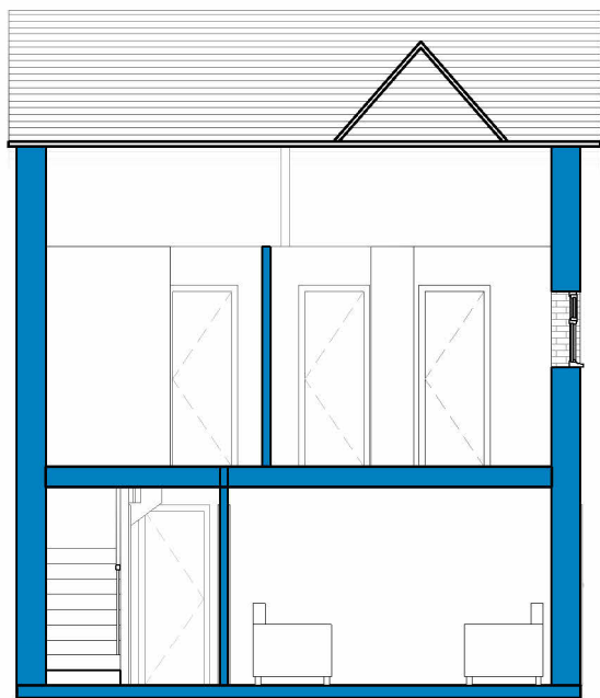
UNIT 3 SECTION
