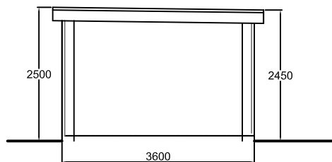
PROPOSED SECTION
