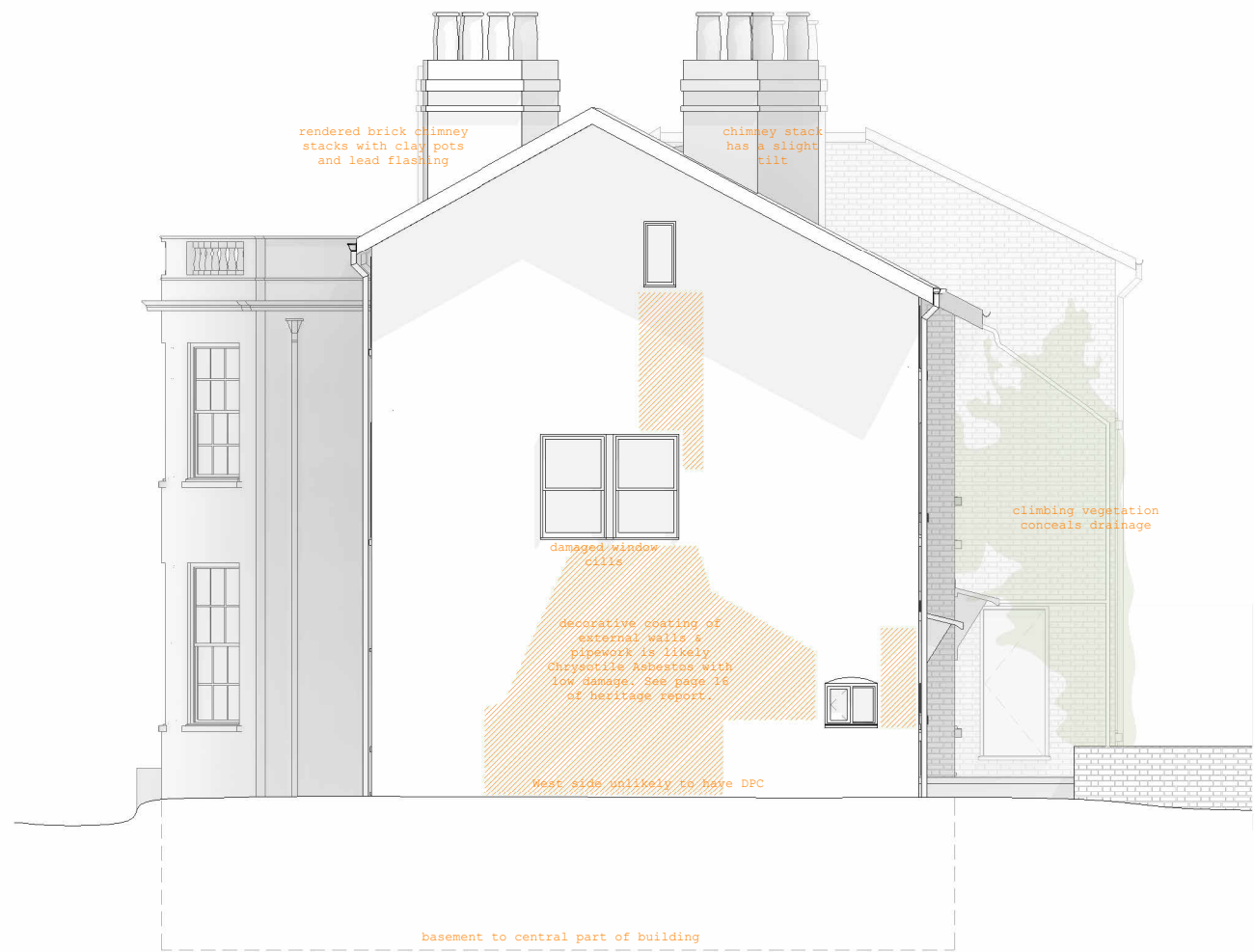
Side Elevation (East)
