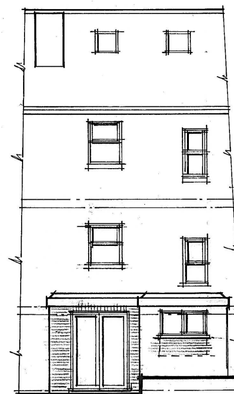
Rear Elevation
