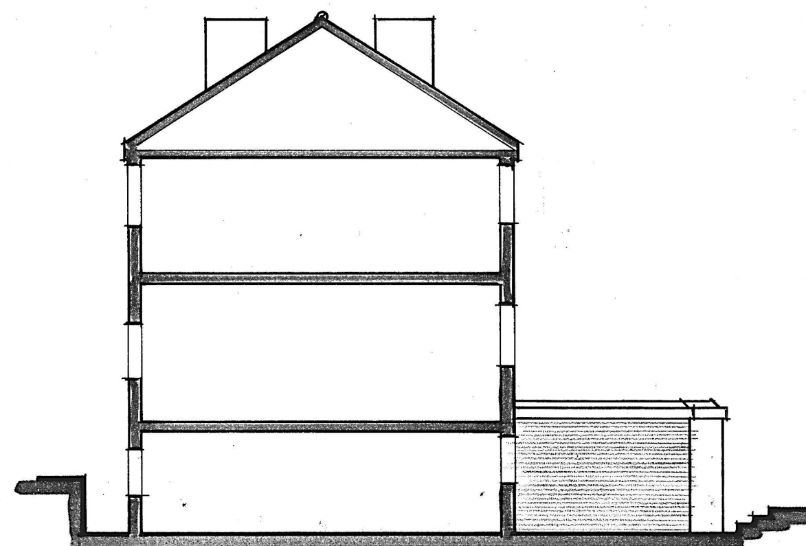
Flank Elevation Scale 1:100
