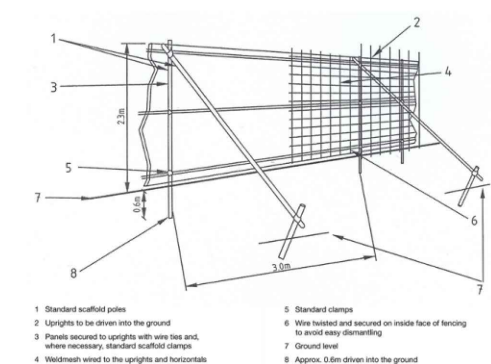
BS:5837 Figure 2 - Tree Protection Fencing structure around RPA
