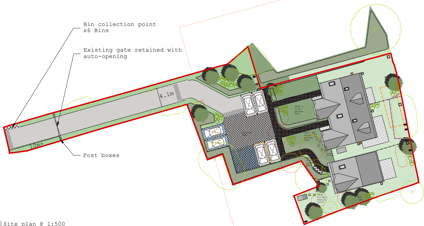
Site plan @ 1:500
