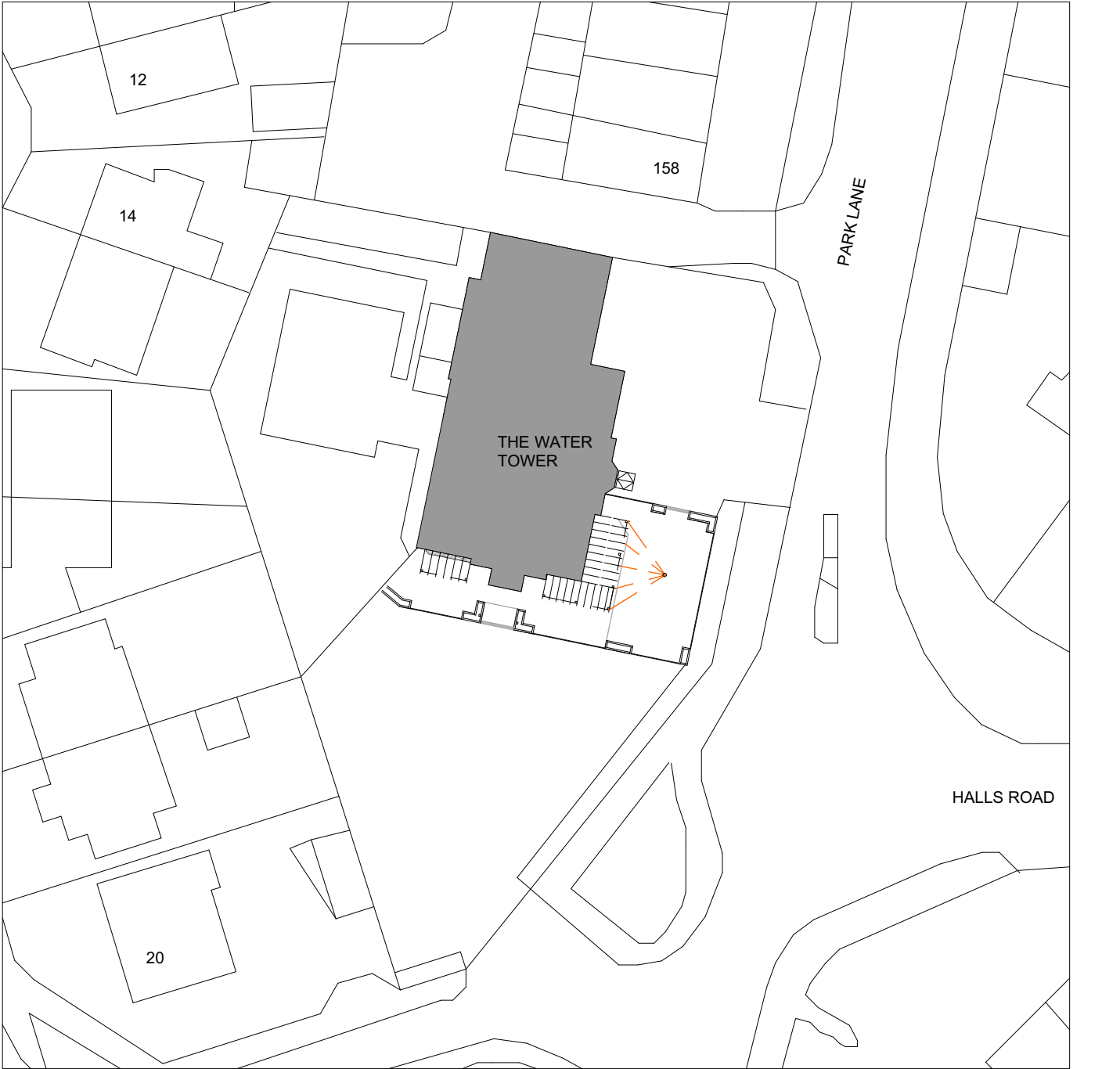
BLOCK PLAN - 1:500 @ A4
