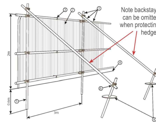
Tree Protection Barrier; details as per Arbicultural Report (section 11.3)
