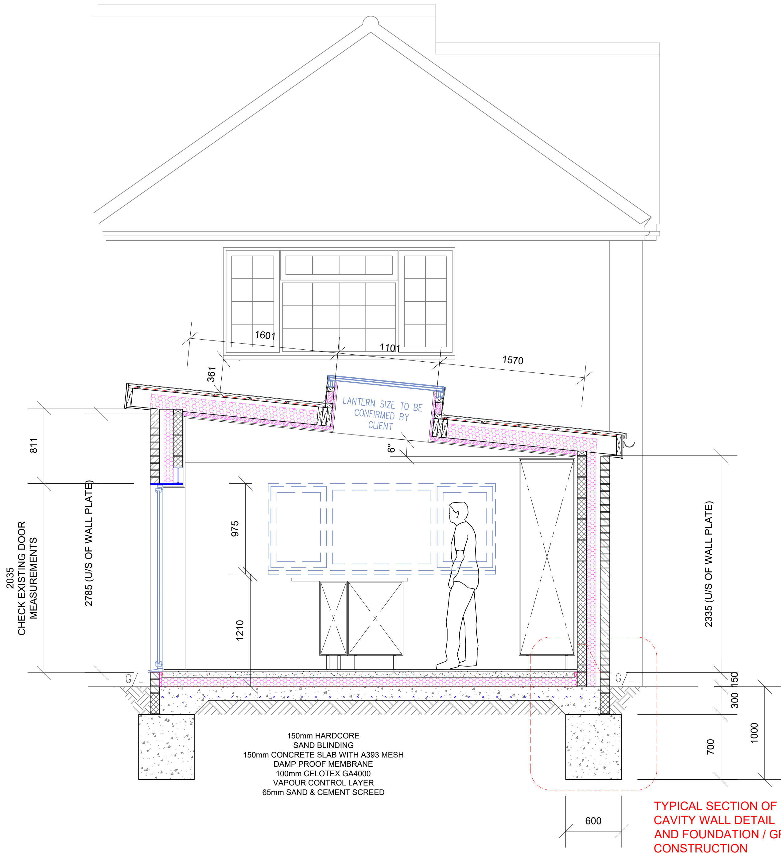
TYPICAL SECTION THROUGH GROUND FLOOR EXTENSION
