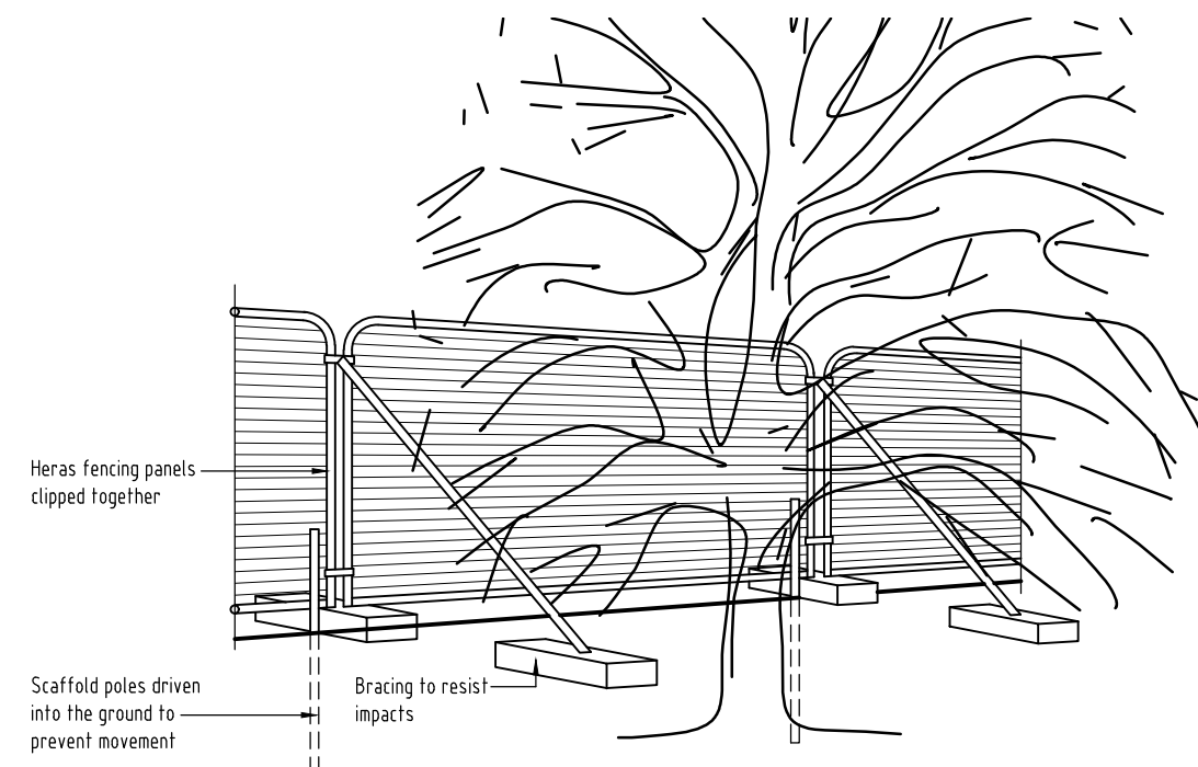
TREE PROTECTION FENCING
