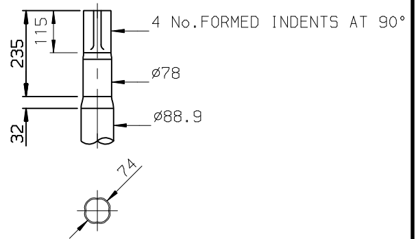
DETAIL OF TOP OF COLUMN. SCALE 1:10
