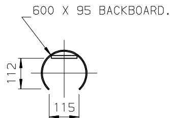
BASE COMPARTMENT. SCALE 1:10
