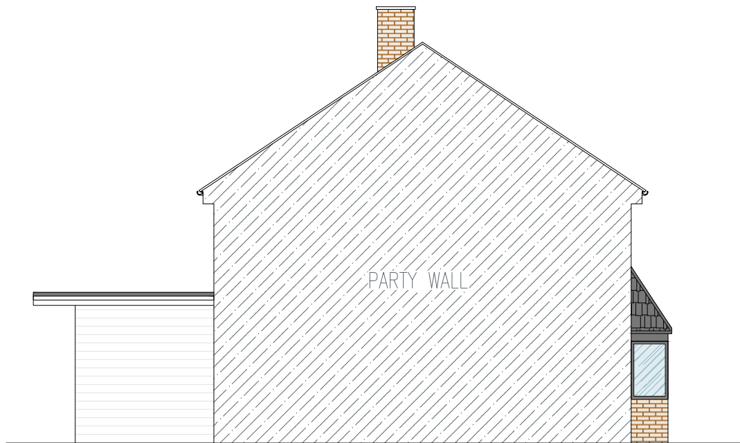
SIDE ELEVATION (NORTH) Sc.1:100
