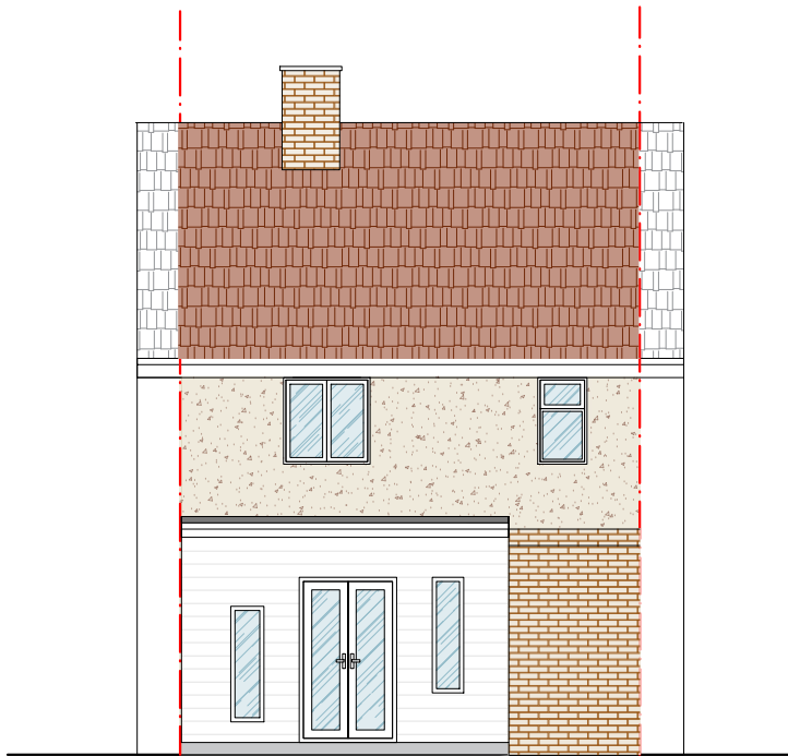
REAR ELEVATION (EAST) Sc.1:100
