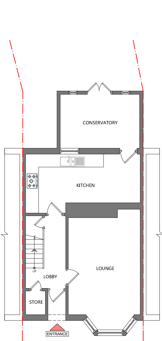
GROUND FLOOR PLAN Sc.1:100
