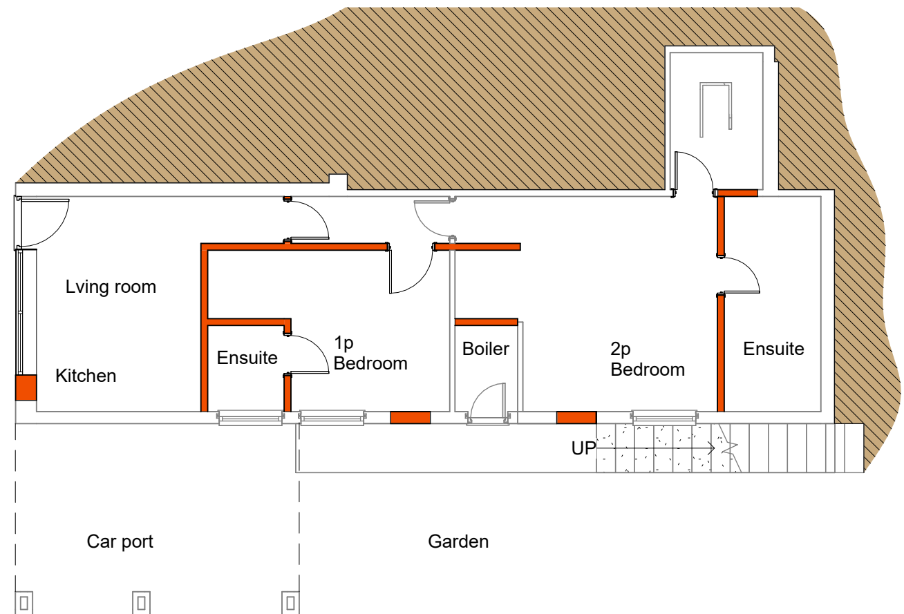
1 Proposed Lower Ground 1 : 100
