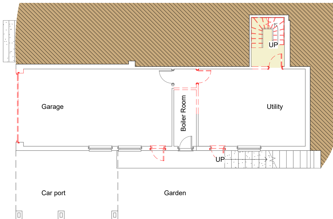
2 Existing Lower Ground 1 : 100
