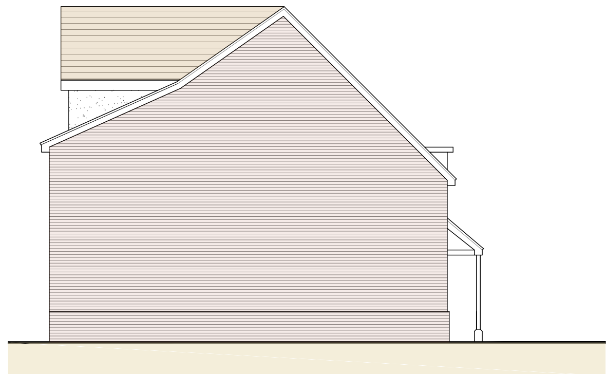
SIDE ELEVATION - PLOT-9 (north east)
