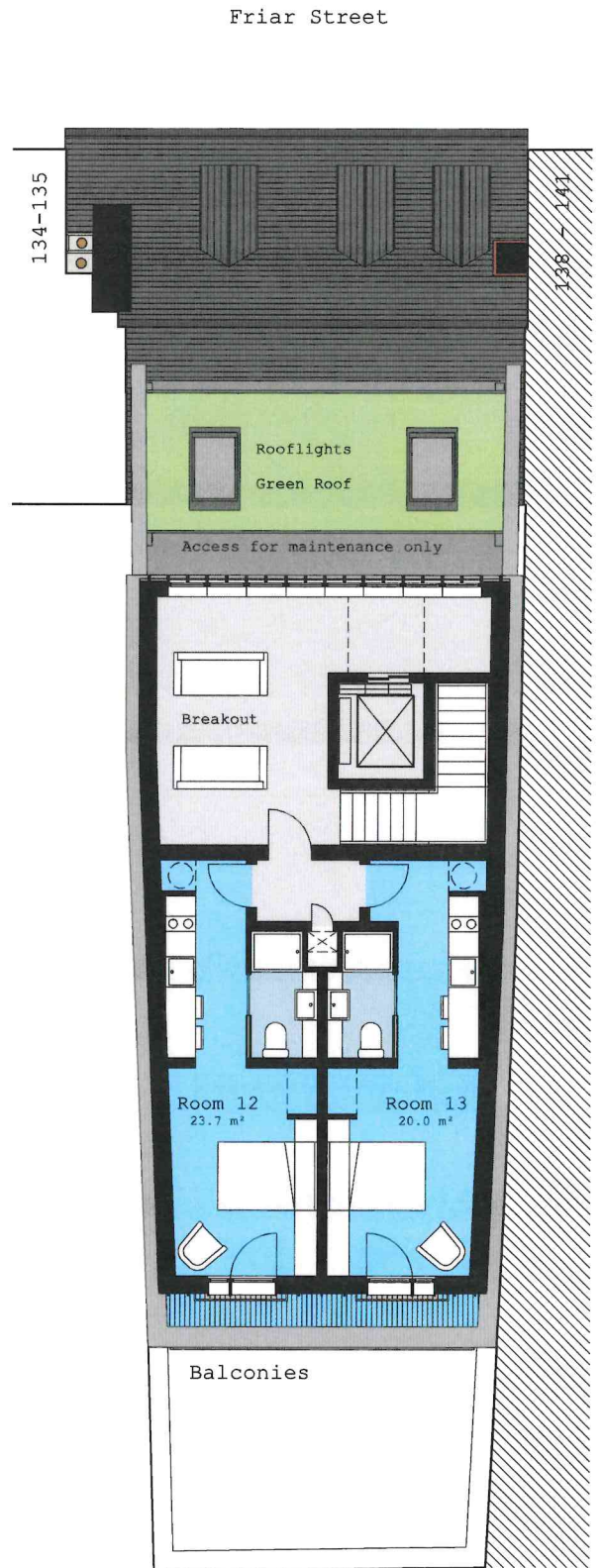
01 Fourth Floor Plan
