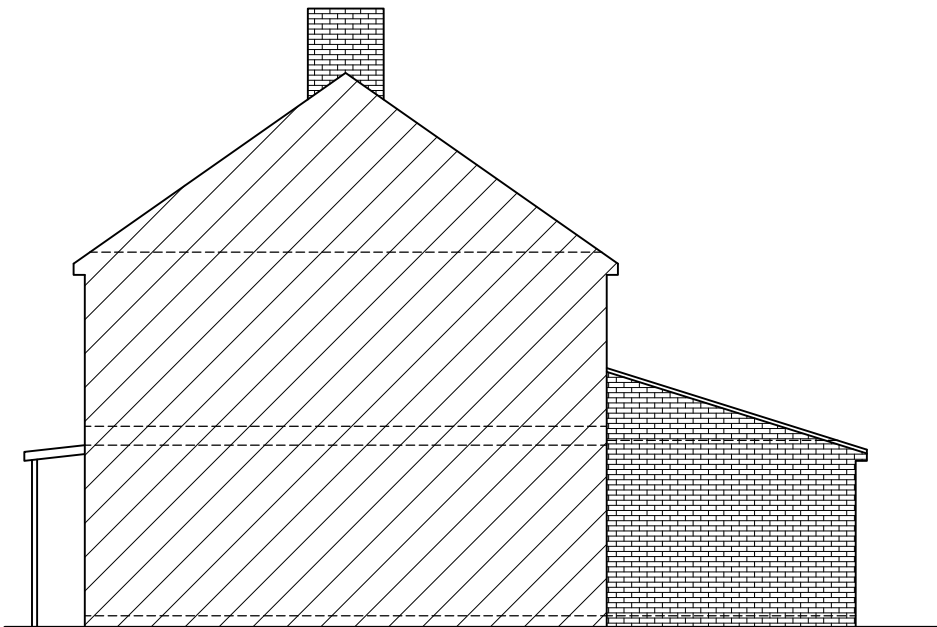
Existing Right Side Elevation Scale: 1/100
