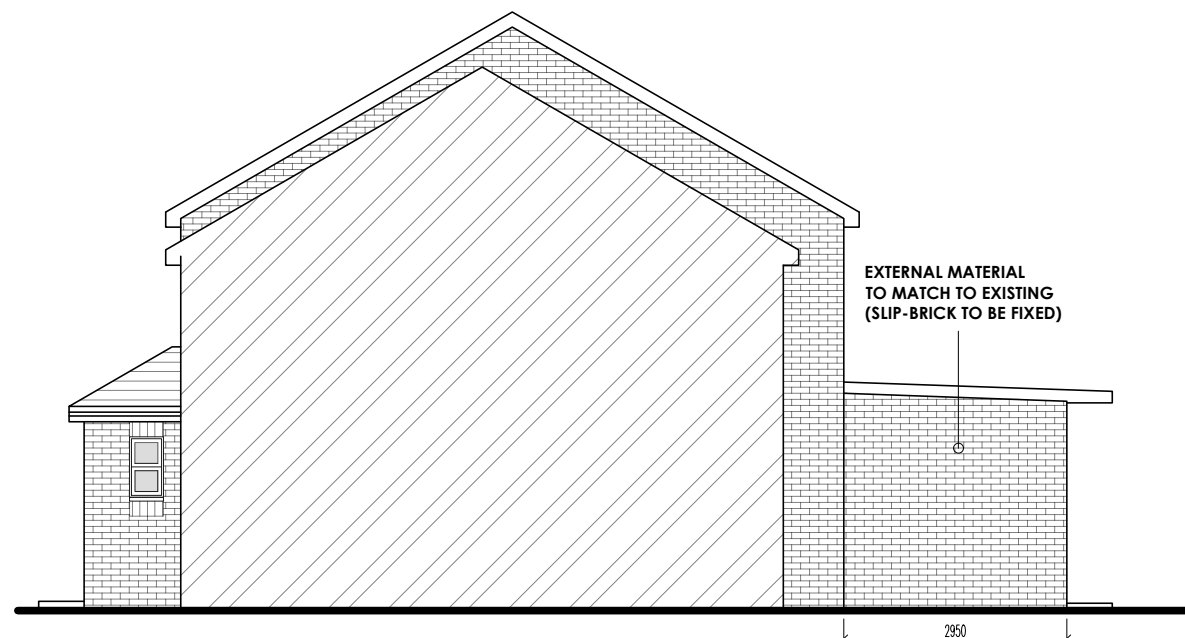
EXISTING SIDE ELEVATION (FROM NO.114) SCALE 1/100
