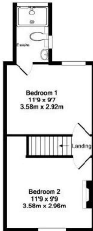
1ST FLOOR APPROX. FLOOR AREA 296 SQ.FT. (27.5 SQ.M.)
