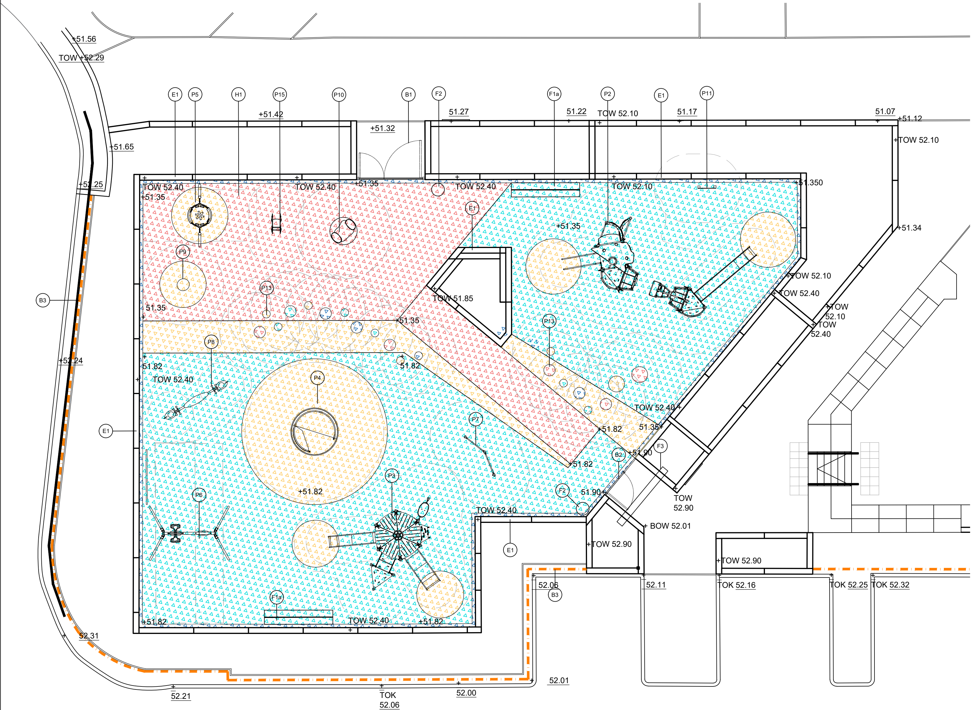
Play Area General Arrangement 1:100@A1
